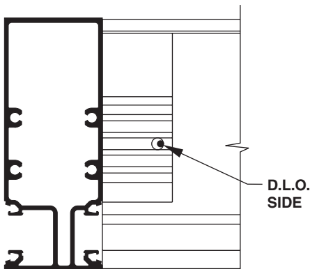
FIGURE 2 FOR FRONT OR BACK OPTION INTERMEDIATE HORIZONTALS
