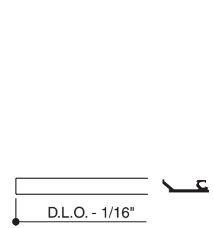
OUTSIDE GLAZED GLASS STOP CUT LENGTH = DLO - 1/16"
