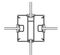
CORNER POST FOUR POCKETS
