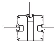
CORNER POST THREE POCKETS
