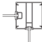
90° OUTSIDE CORNER TWO POCKETS
